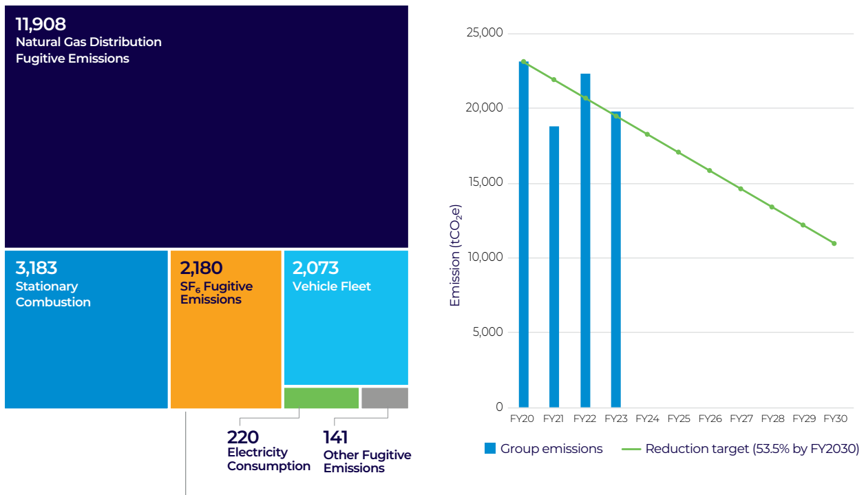
Figure 5: Emissions included in vector's science-aligned target - Scope 1 and 2 excluding distribution losses. (left) Emission breakdown in tCO 2 e. (right) Vector's trajectory towards its 53.5% emission reduction target.
